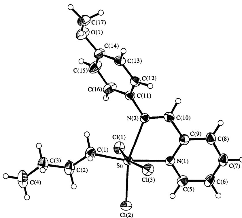
Fig. 1. Molecular structure with atom labelling for n\text{-BuSnCl}_3[\text{C}_5\text{H}_4\text{NC}(\text{H})=\text{NC}_6\text{H}_3\text{OCH}_3\text{-}p] .
